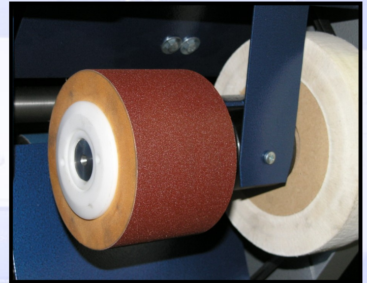
Birki Wheel for bottom scouring
