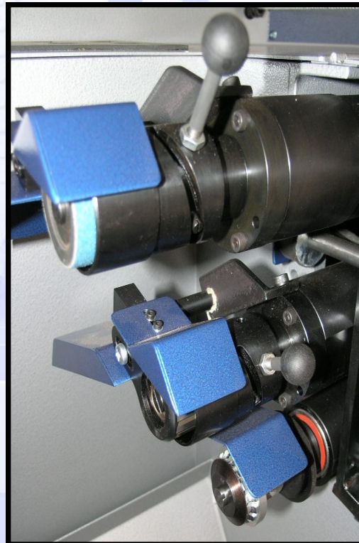
710 fitted with 3rd head and top-piece scouring roll
