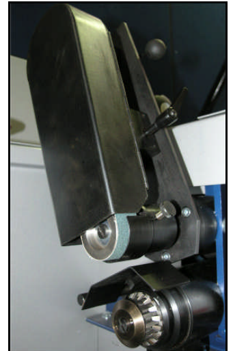
Improved mini band unit and adjustable forepart cutter
